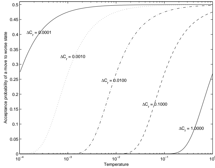
Figure 4: Acceptance probability curves for the normalized inverse exponential function (6) with q = 0.95 . The curves represent constant values of \Delta C_r = \frac{\Delta C}{C_0} . Probability of moving to a worse state decreases when the temperature decreases. Moves to slightly worse state have higher probability than those with large degradation.
