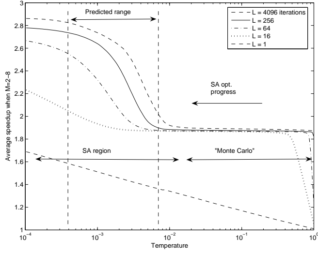
Figure 5: Averaged speedup with respect to temperature for 300 node graphs with different L values. The temperature range given with (18)(19) k = 1 is labeled “predicted range”. Notice that temperature and the number of iterations increase in different directions. The number of mapping iterations increases as the temperature decreases.
