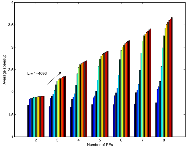
Figure 6: Averaged speedups for 300 node graphs with M=2-8 processing elements and different L values ( L = 1, 2, 4, \dots, 4096 ) for each processing element set.
