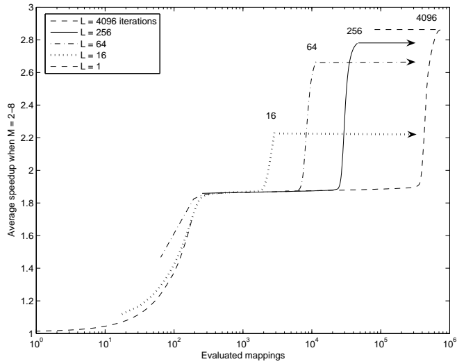
Figure 7: Averaged speedup with respect to mapping evaluations for 300 node graphs with different L values.
